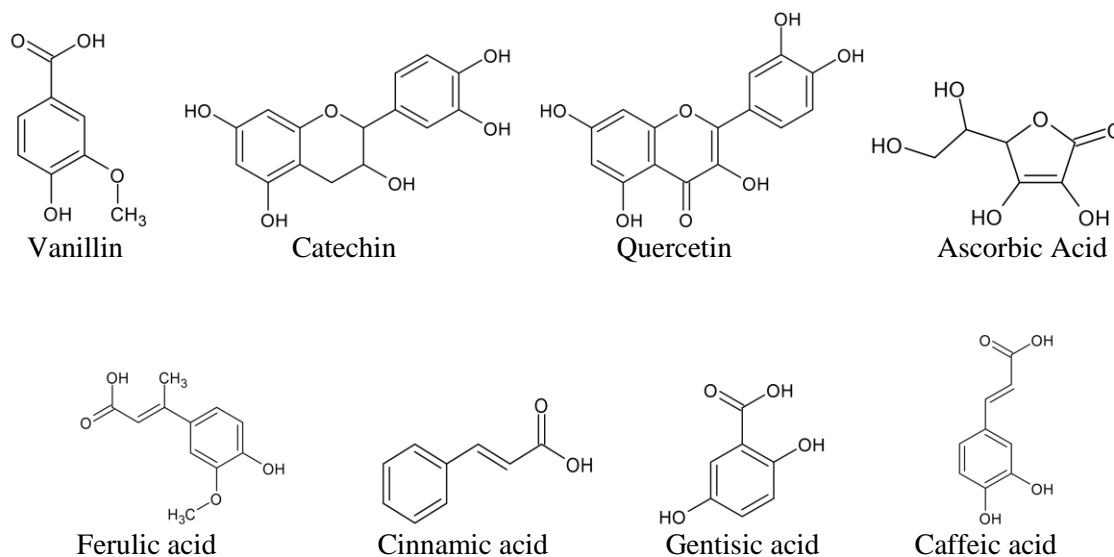
Chemical structures of some nutraceutical compounds
