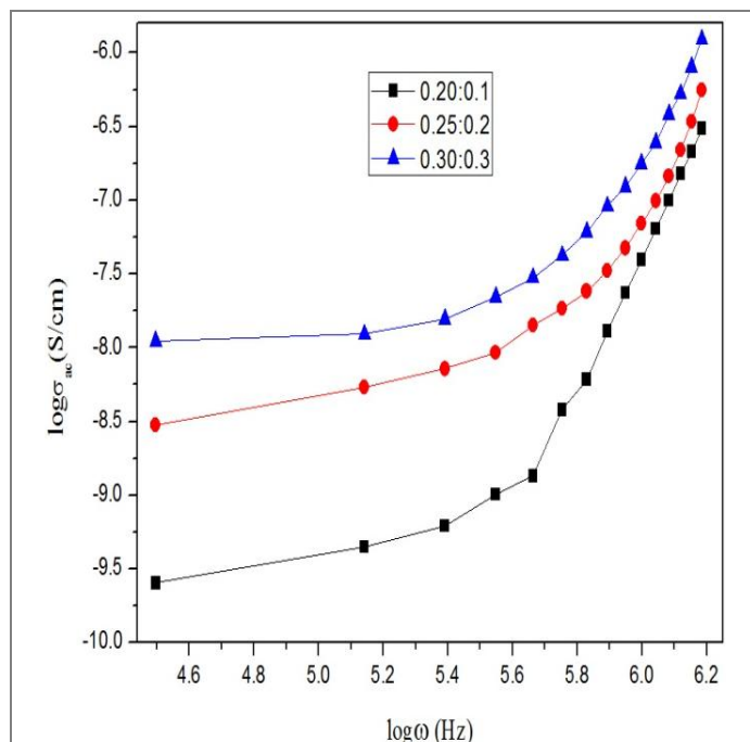
Figure 4 Variation of \log \sigma with with logarithmic conductivity for different wt% ratios
