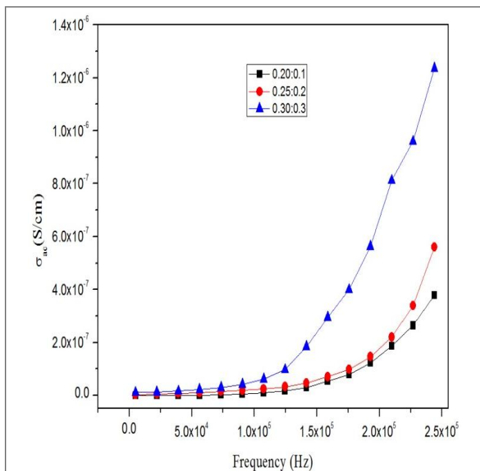
Figure 3 Variation of the ionic conductivity frequency for different wt% ratios
