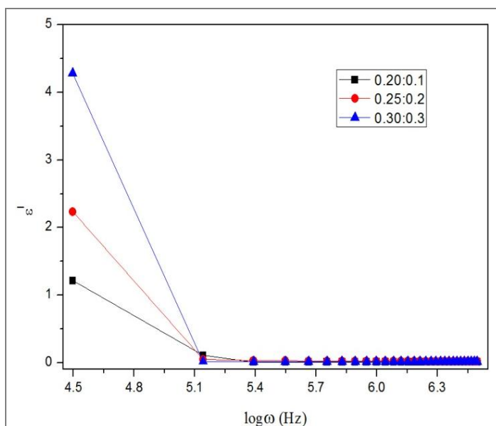
Figure 5 Variation of dielectric constant real part ( \epsilon' ) with the logarithmic angular frequency for different wt% ratios
