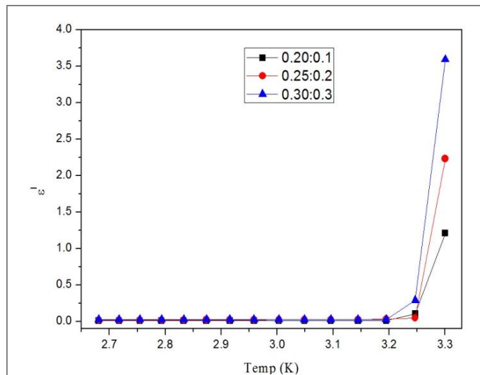
Figure 8 Variation of temperature with dielectric constant real part ( \epsilon' ) for different wt% ratios
