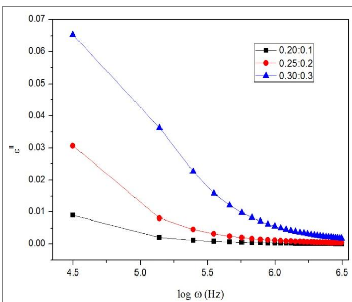
Figure 6 Variation of dielectric constant imaginary part ( \epsilon'' ) with the logarithmic angular frequency for different wt% ratios
